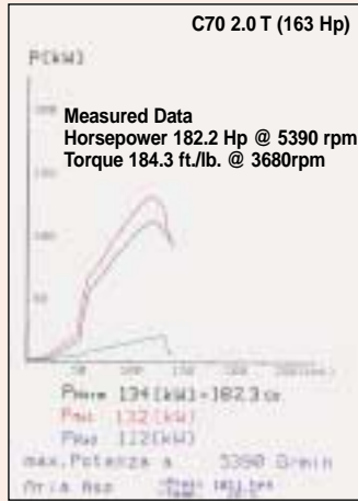
SUPERSPRINT: - CENTER PIPE + REAR MUFFLER 331805
